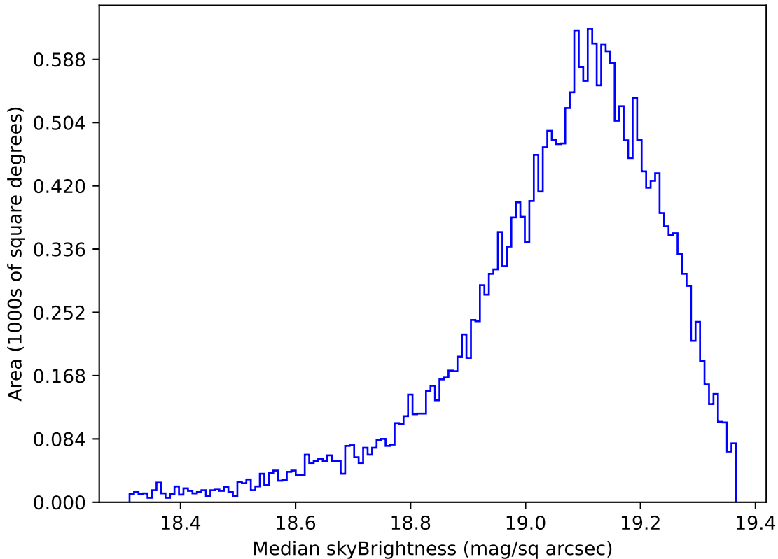
ddf_acor_sf25_lsf40_lsr10_v3.4_10yrs Yr 1 z band: Median skyBrightness
