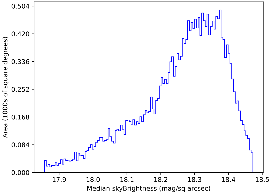
ddf_acor_sf25_lsf40_lsr10_v3.4_10yrs Yr 1 y band: Median skyBrightness
