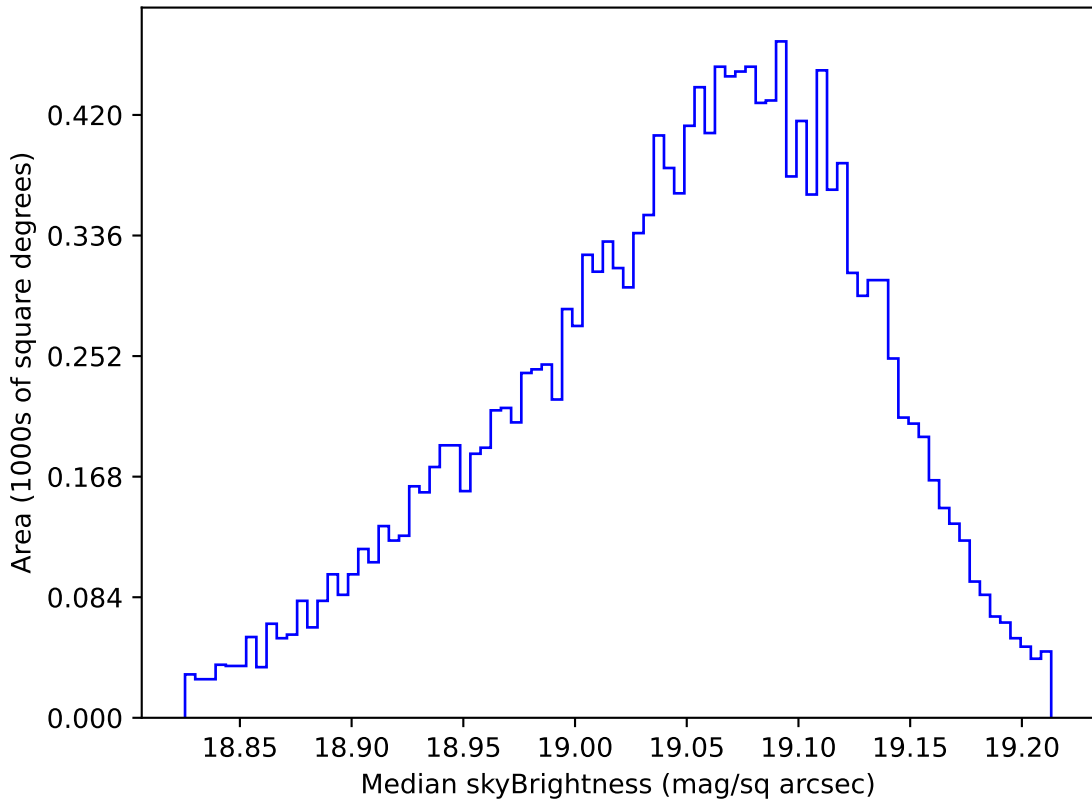
ddf_acor_sf25_lsf40_lsr10_v3.4_10yrs WFD z band: Median skyBrightness
