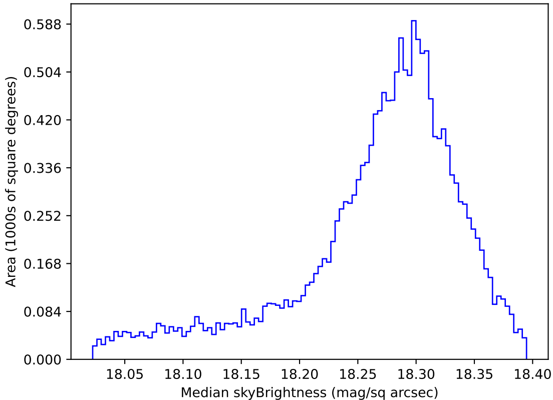
ddf_acor_sf25_lsf40_lsr10_v3.4_10yrs WFD y band: Median skyBrightness
