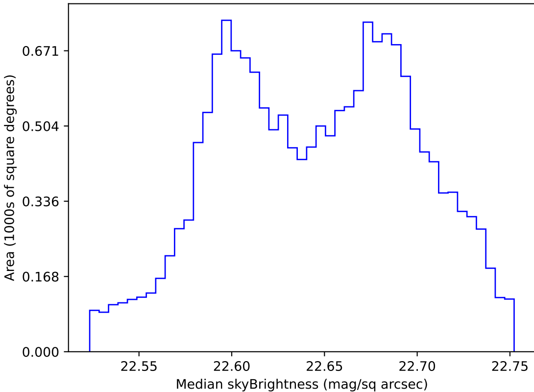
ddf_acor_sf25_lsf40_lsr10_v3.4_10yrs WFD u band: Median skyBrightness
