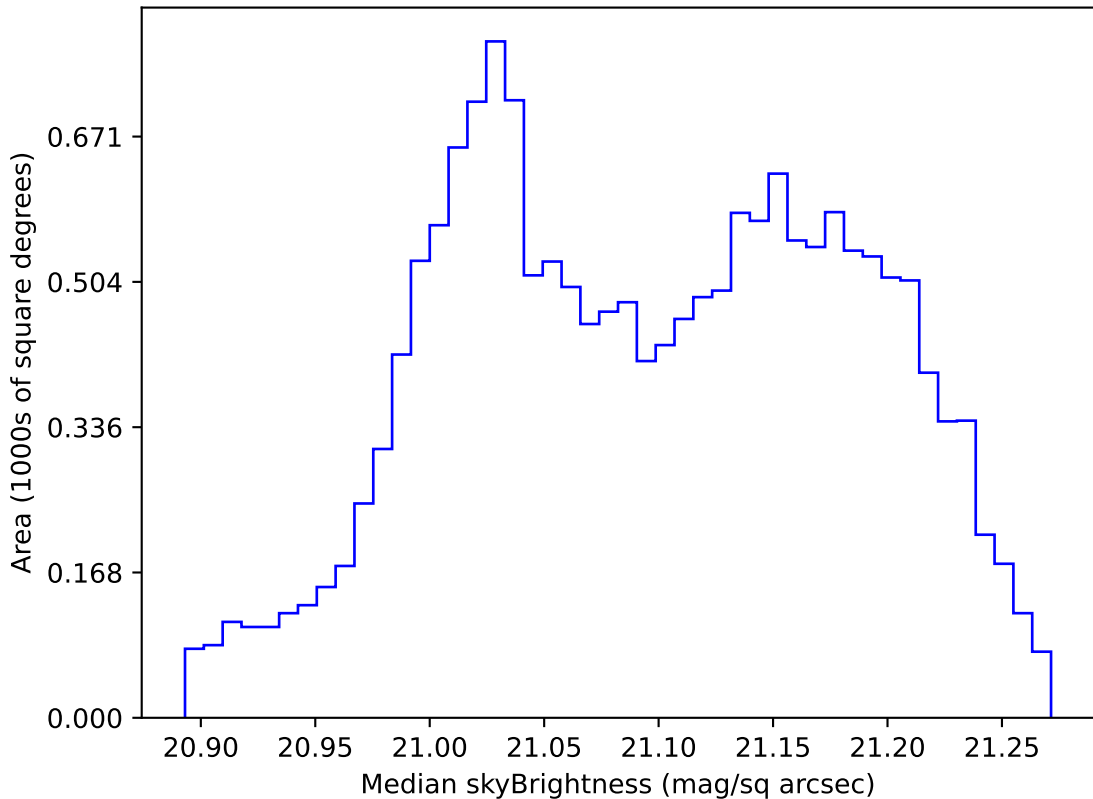
ddf_acor_sf25_lsf40_lsr10_v3.4_10yrs WFD r band: Median skyBrightness
