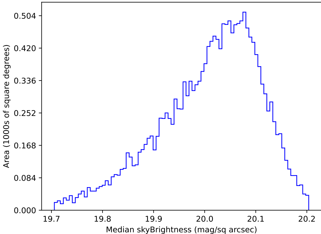
ddf_acor_sf25_lsf40_lsr10_v3.4_10yrs WFD i band: Median skyBrightness
