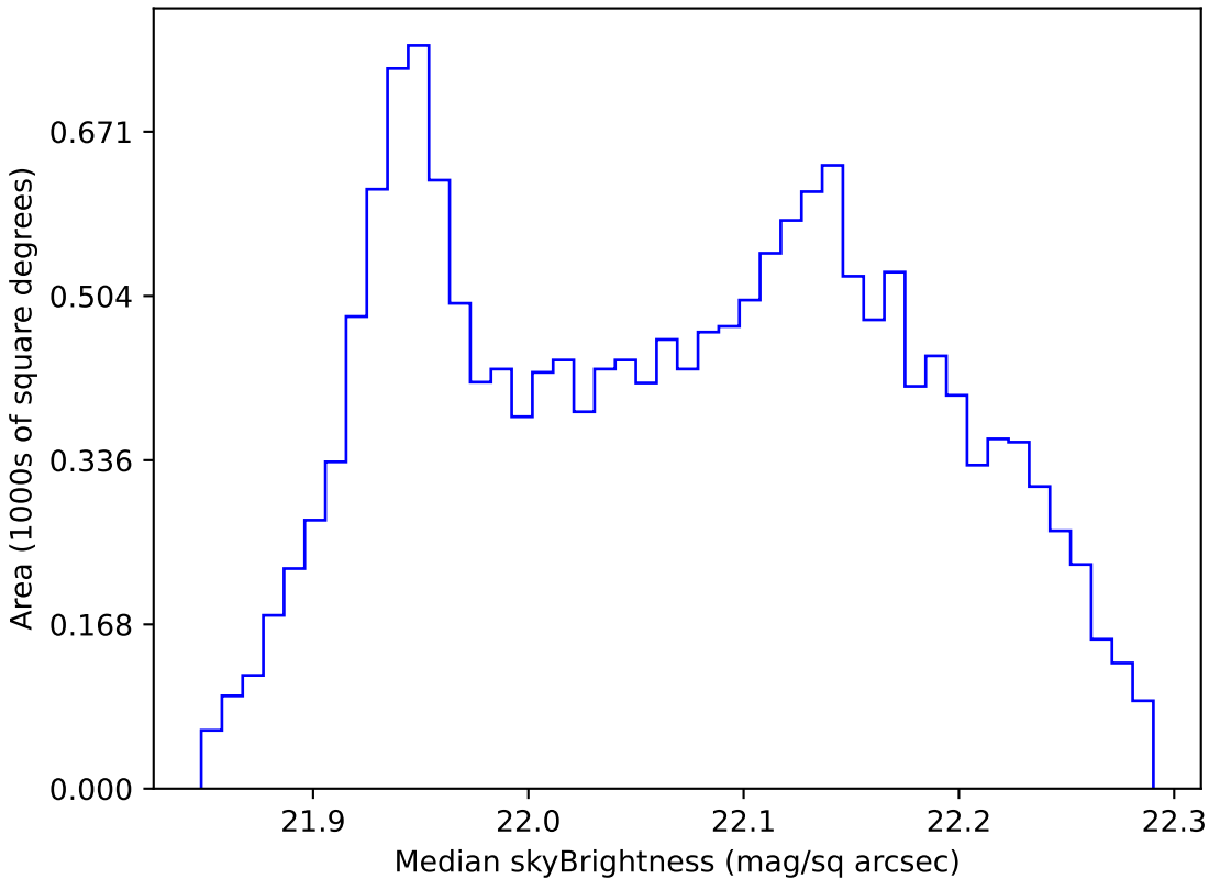
ddf_acor_sf25_lsf40_lsr10_v3.4_10yrs WFD g band: Median skyBrightness
