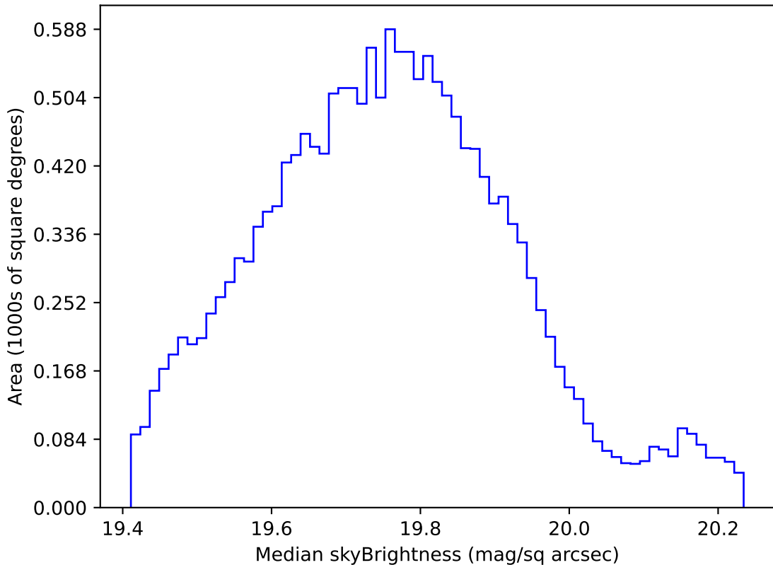
ddf_acor_sf25_lsf40_lsr10_v3.4_10yrs WFD all bands: Median skyBrightness
