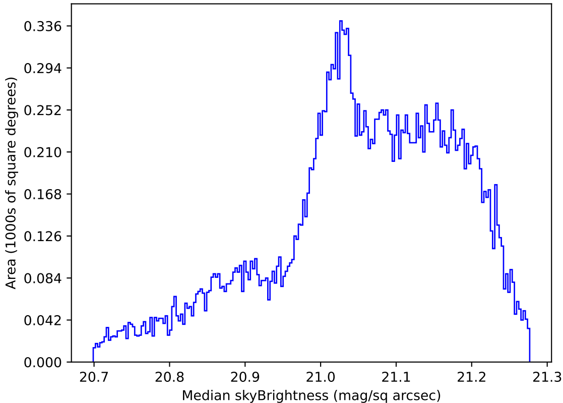
ddf_acor_sf25_lsf40_lsr10_v3.4_10yrs All sky r band: Median skyBrightness
