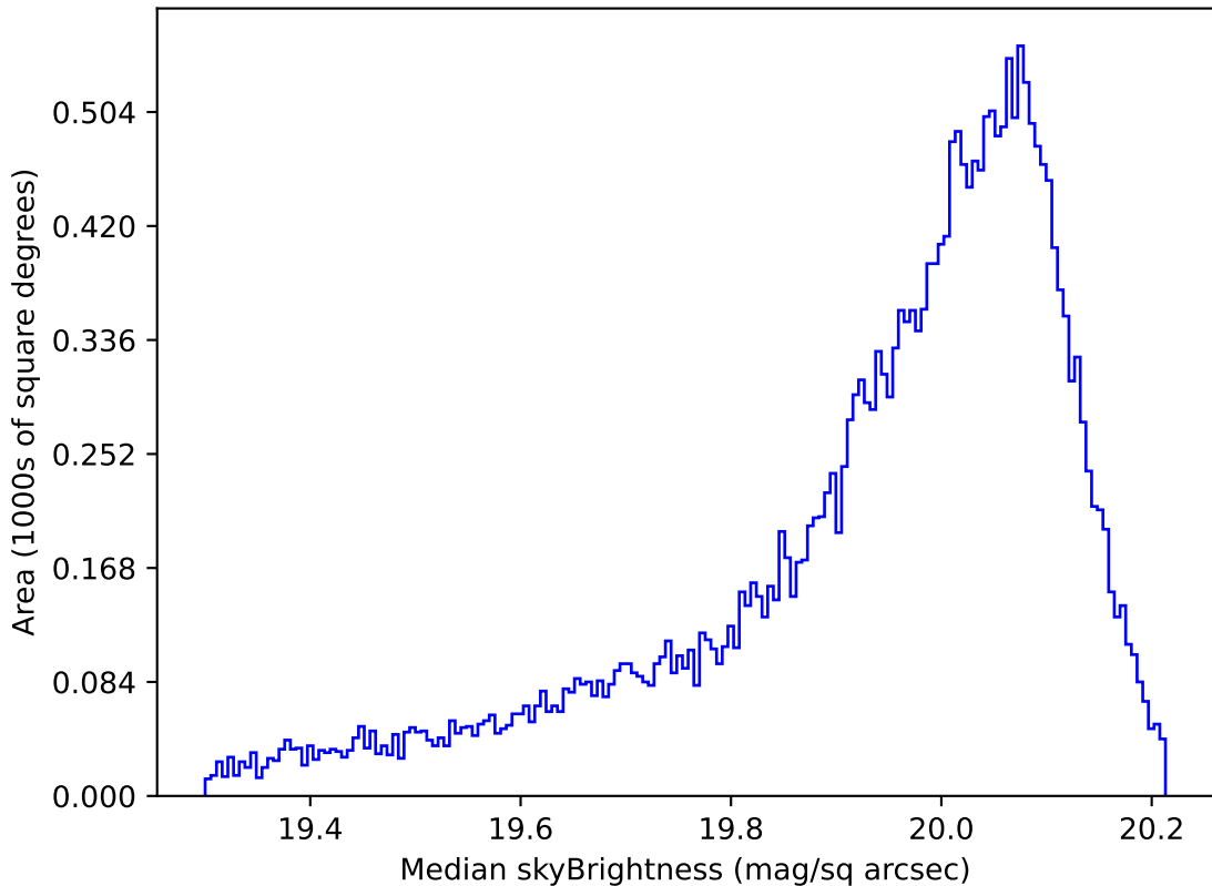
ddf_acor_sf25_lsf40_lsr10_v3.4_10yrs All sky i band: Median skyBrightness
