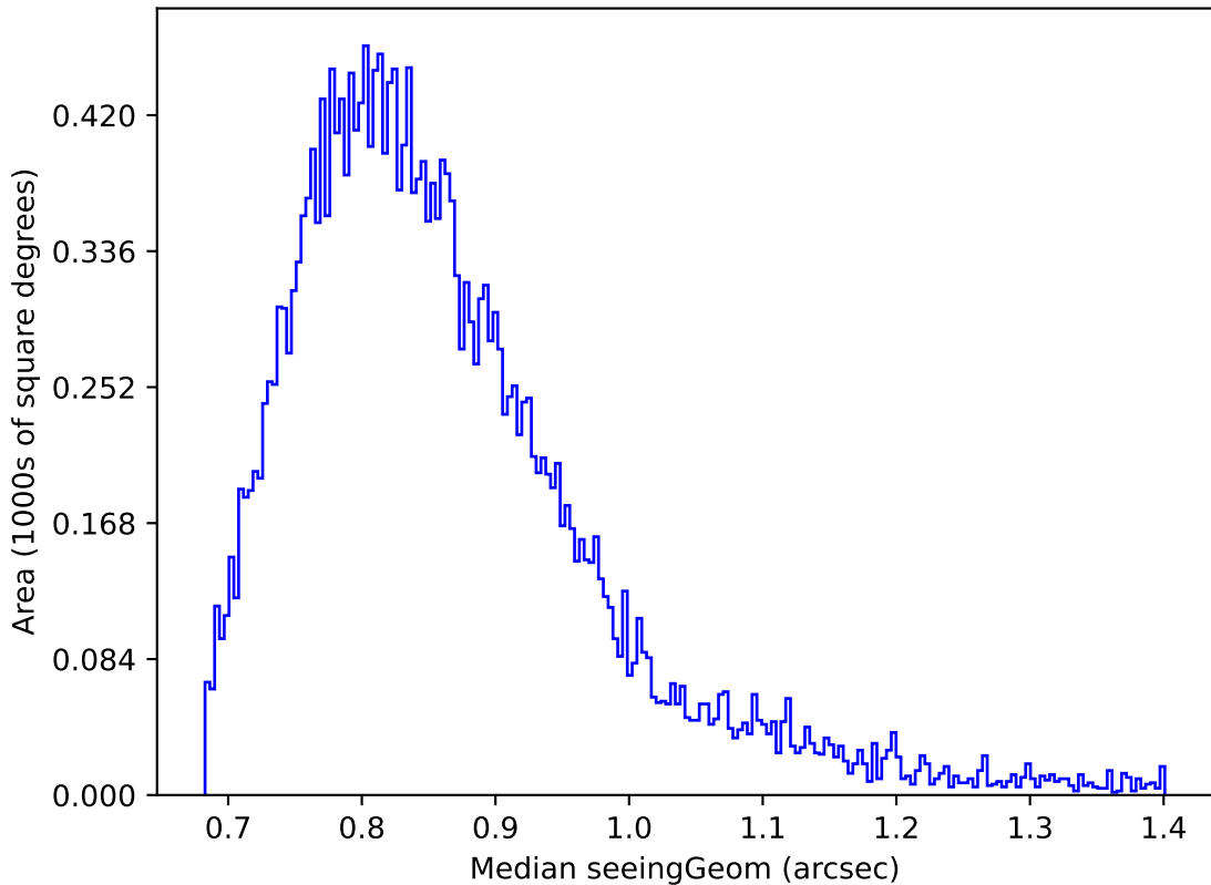
ddf_acor_sf25_lsf40_lsr10_v3.4_10yrs Yr 1 z band: Median seeingGeom
