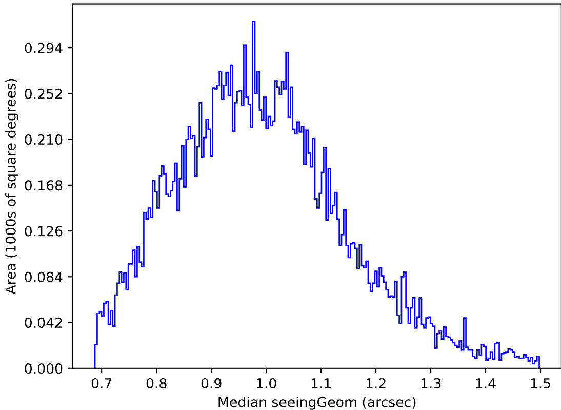
ddf_acor_sf25_lsf40_lsr10_v3.4_10yrs Yr 1 u band: Median seeingGeom
