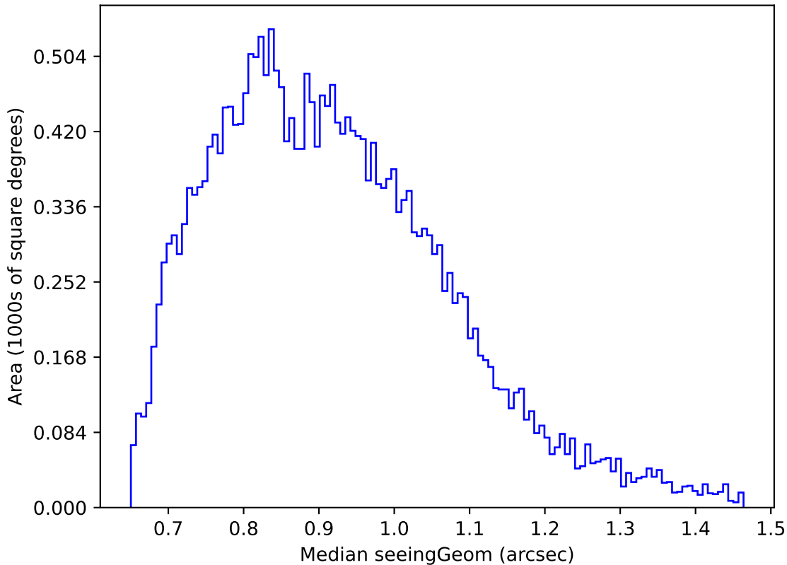
ddf_acor_sf25_lsf40_lsr10_v3.4_10yrs Yr 1 g band: Median seeingGeom
