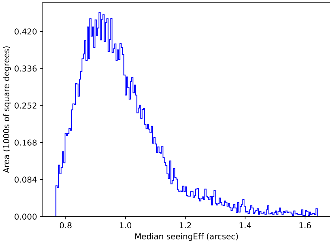
ddf_acor_sf25_lsf40_lsr10_v3.4_10yrs Yr 1 z band: Median seeingEff
