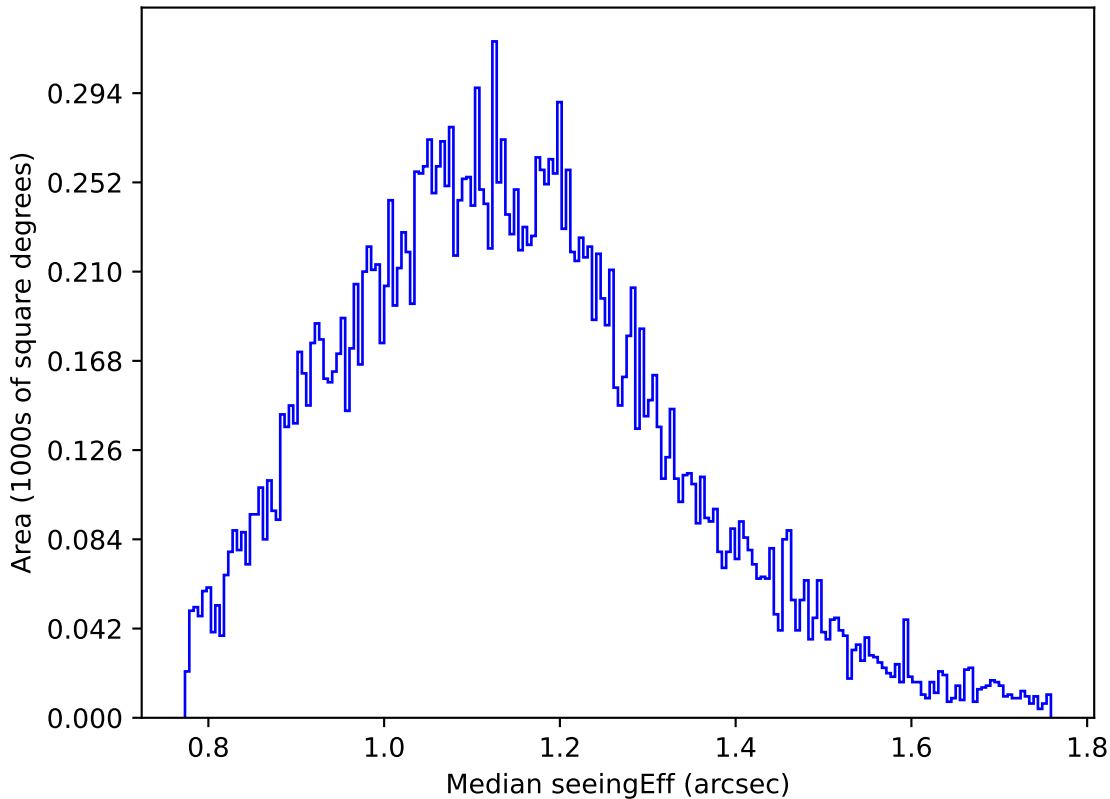
ddf_acor_sf25_lsf40_lsr10_v3.4_10yrs Yr 1 u band: Median seeingEff
