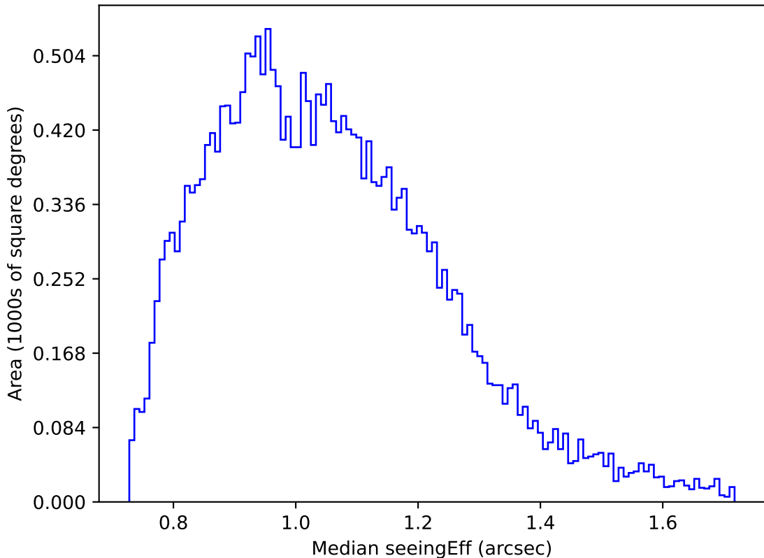
ddf_acor_sf25_lsf40_lsr10_v3.4_10yrs Yr 1 g band: Median seeingEff
