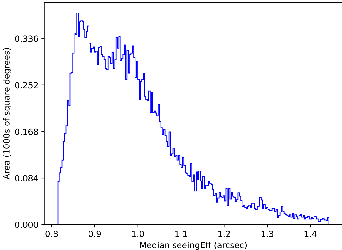
ddf_acor_sf25_lsf40_lsr10_v3.4_10yrs Yr 1 all bands: Median seeingEff
