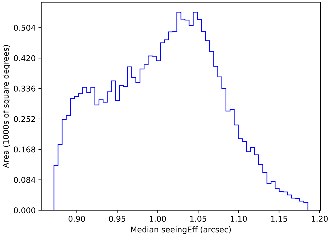
ddf_acor_sf25_lsf40_lsr10_v3.4_10yrs WFD z band: Median seeingEff
