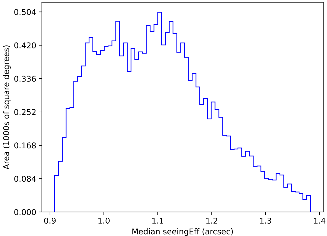
ddf_acor_sf25_lsf40_lsr10_v3.4_10yrs WFD g band: Median seeingEff
