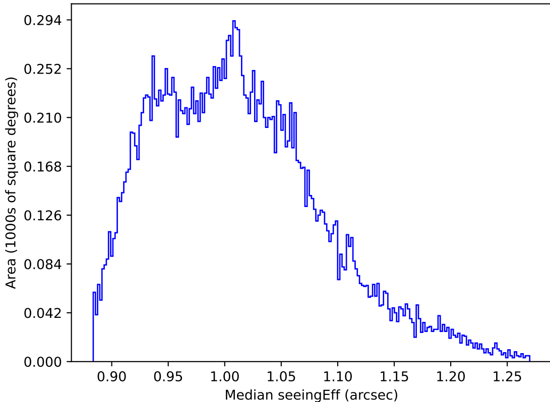
ddf_acor_sf25_lsf40_lsr10_v3.4_10yrs All sky y band: Median seeingEff
