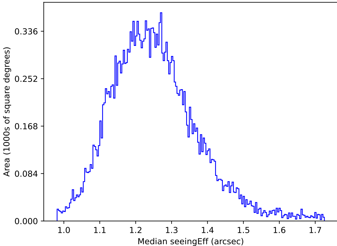
ddf_acor_sf25_lsf40_lsr10_v3.4_10yrs All sky u band: Median seeingEff
