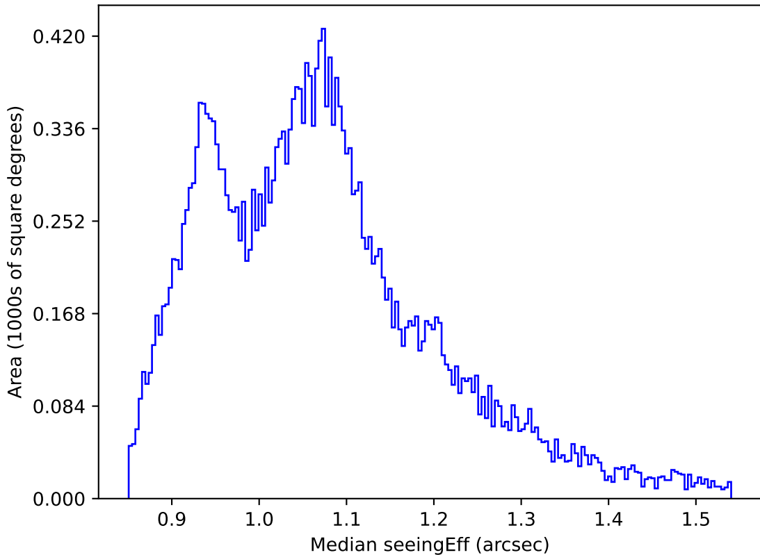
ddf_acor_sf25_lsf40_lsr10_v3.4_10yrs All sky r band: Median seeingEff
