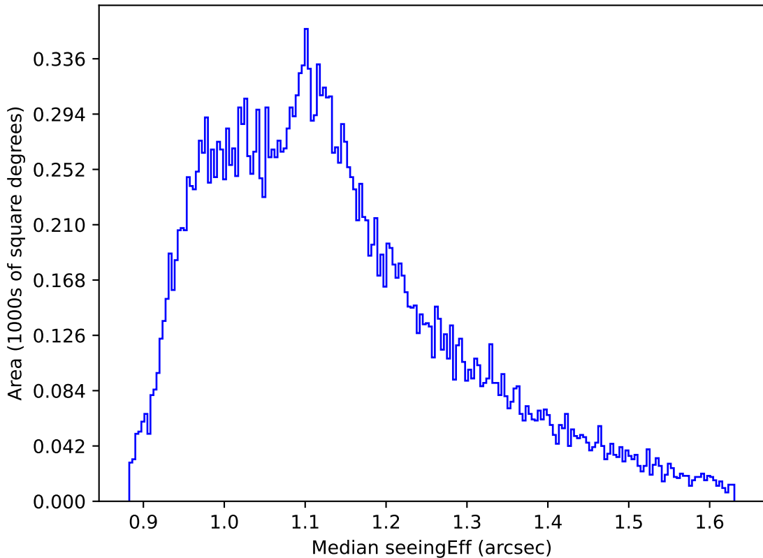
ddf_acor_sf25_lsf40_lsr10_v3.4_10yrs All sky g band: Median seeingEff
