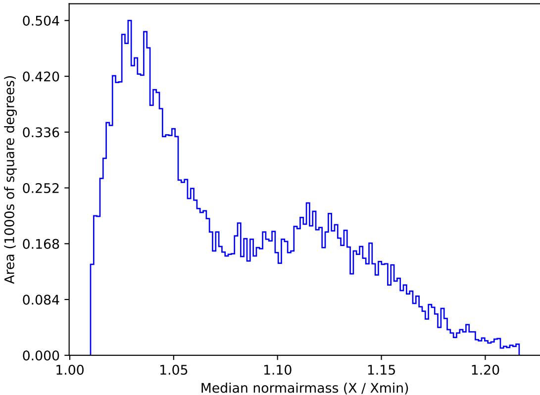
ddf_acor_sf25_lsf40_lsr10_v3.4_10yrs All sky u band: Median normairmass
