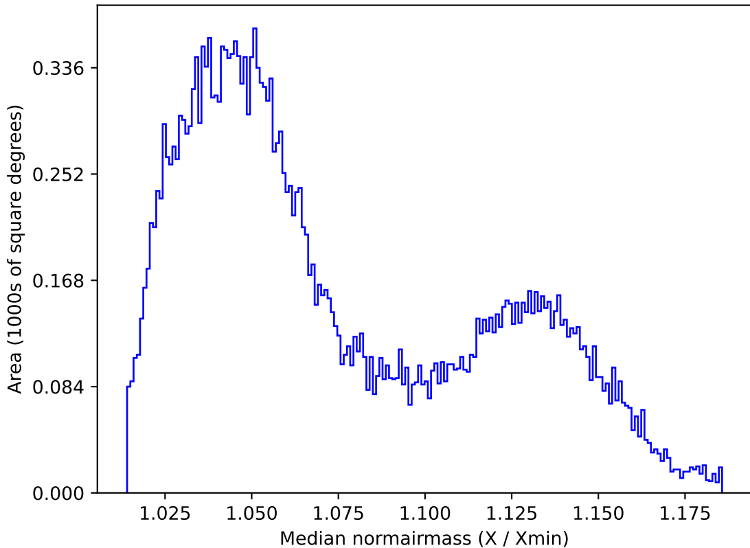
ddf_acor_sf25_lsf40_lsr10_v3.4_10yrs All sky r band: Median normairmass
