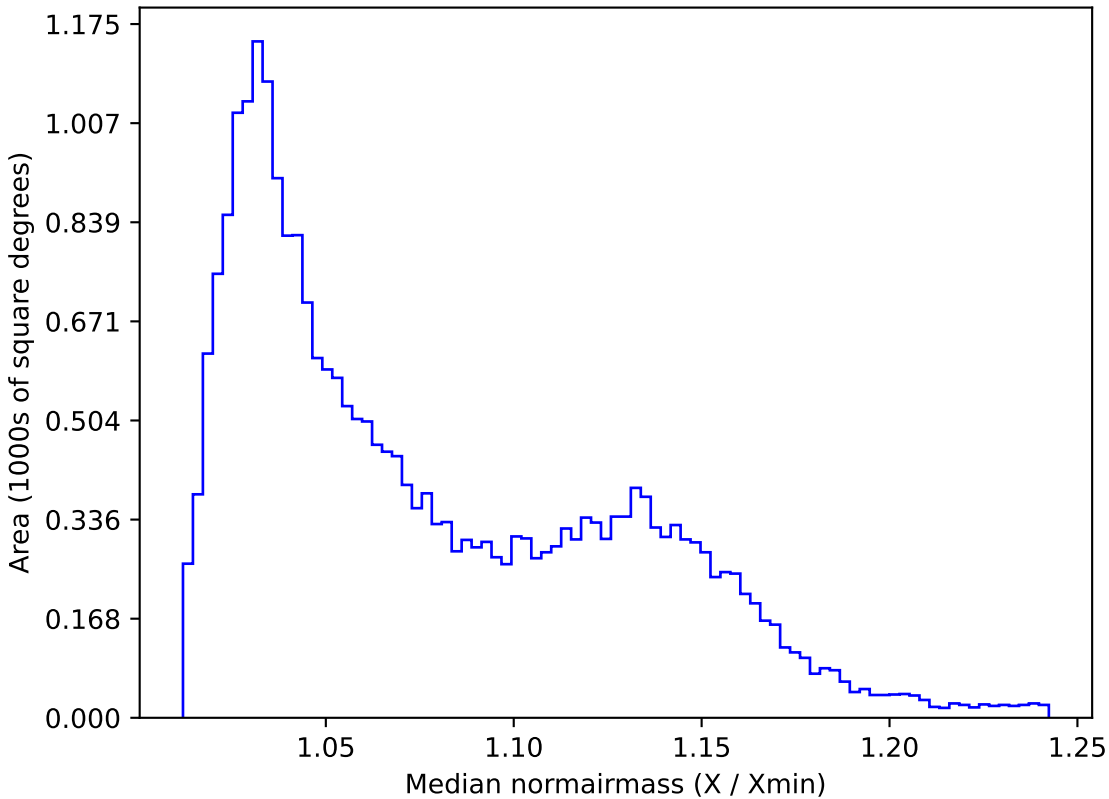
ddf_acor_sf25_lsf40_lsr10_v3.4_10yrs All sky g band: Median normairmass
