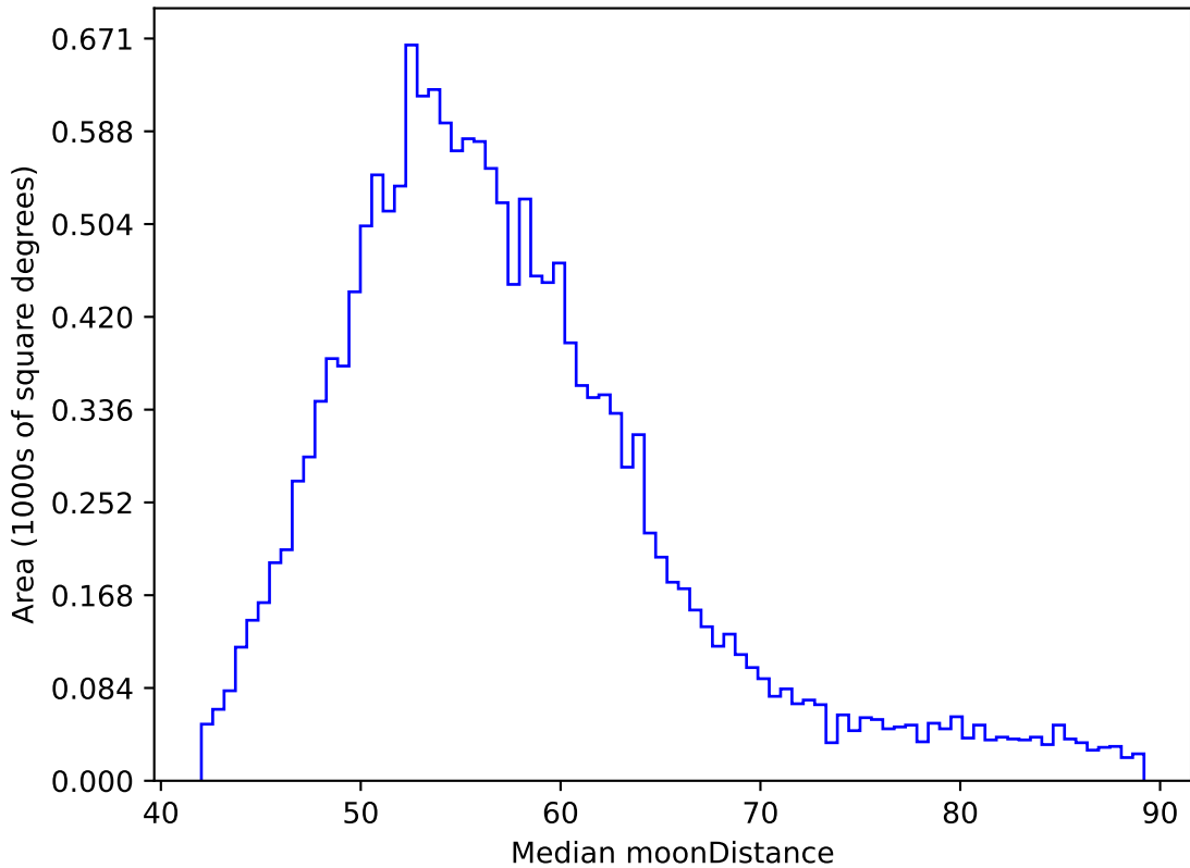
ddf_acor_sf25_lsf40_lsr10_v3.4_10yrs WFD y band: Median moonDistance
