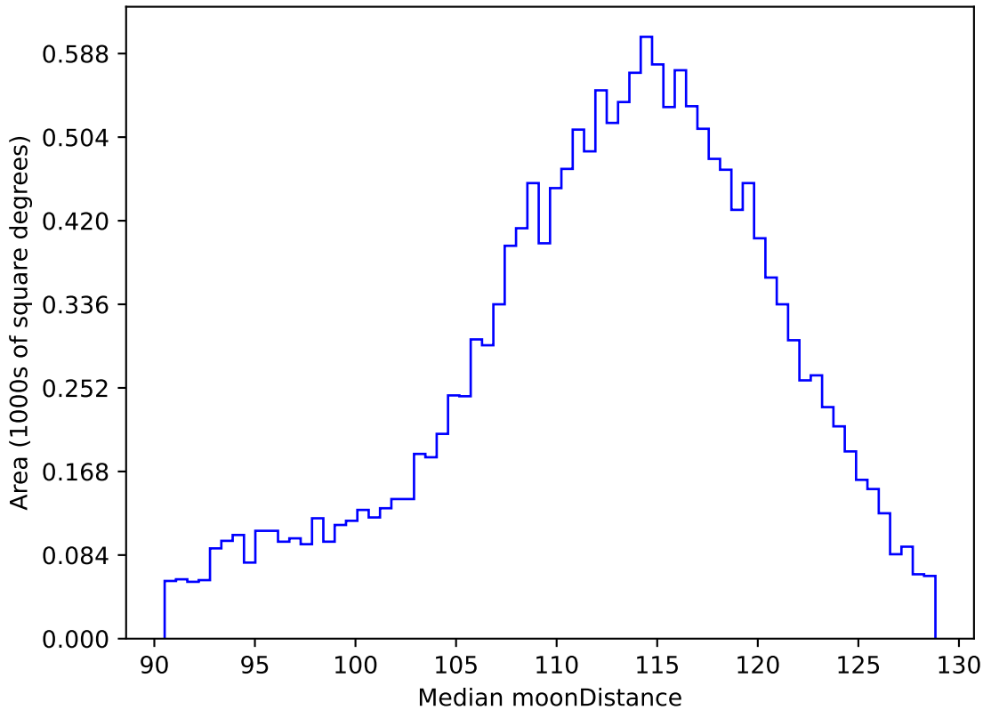
ddf_acor_sf25_lsf40_lsr10_v3.4_10yrs WFD r band: Median moonDistance
