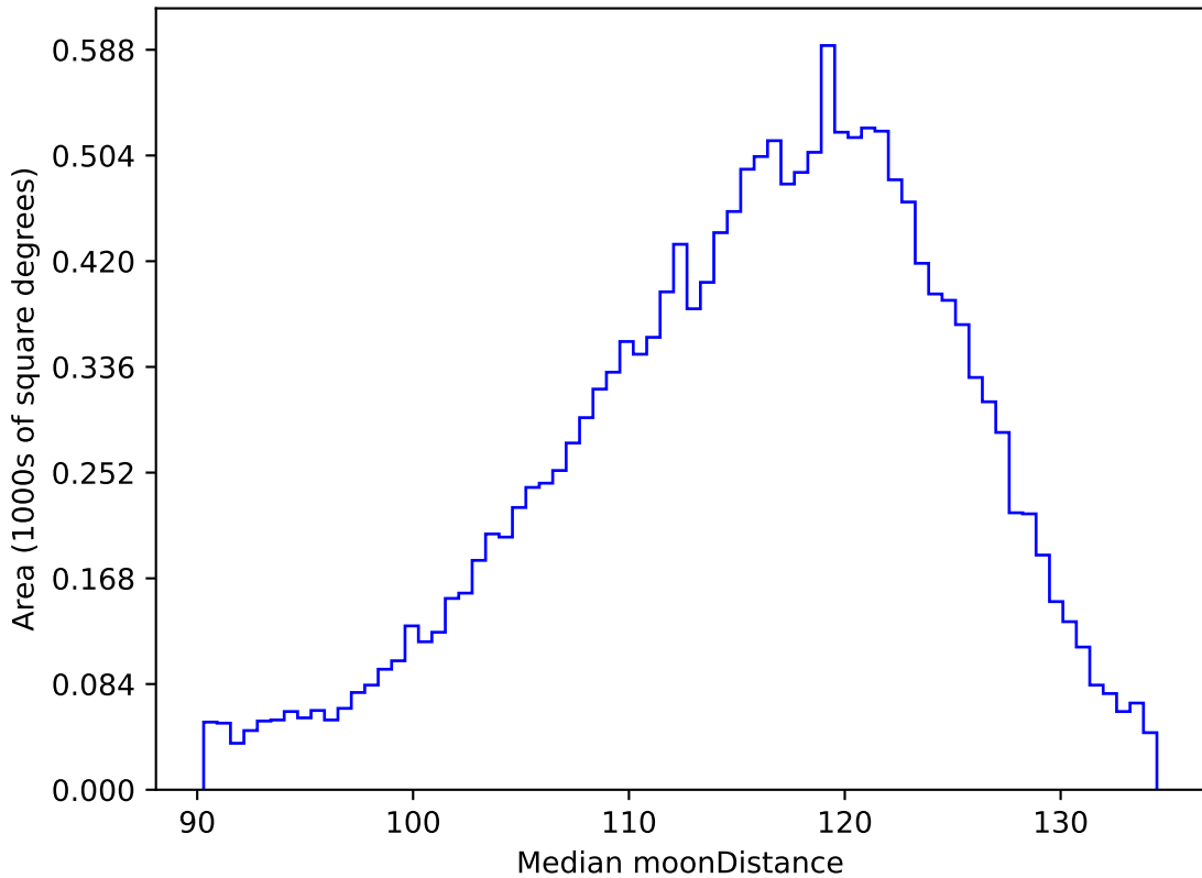
ddf_acor_sf25_lsf40_lsr10_v3.4_10yrs WFD g band: Median moonDistance
