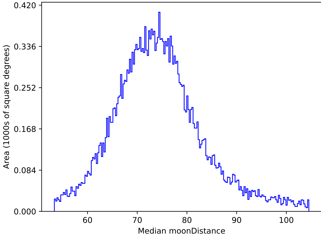
ddf_acor_sf25_lsf40_lsr10_v3.4_10yrs All sky z band: Median moonDistance
