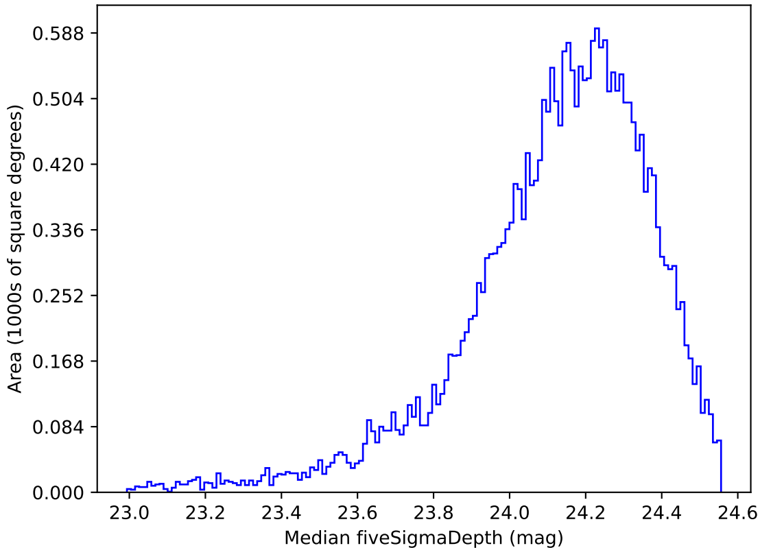
ddf_acor_sf25_lsf40_lsr10_v3.4_10yrs Yr 1 r band: Median fiveSigmaDepth
