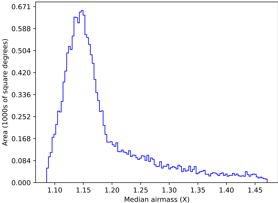
ddf_acor_sf25_lsf40_lsr10_v3.4_10yrs WFD z band: Median airmass
