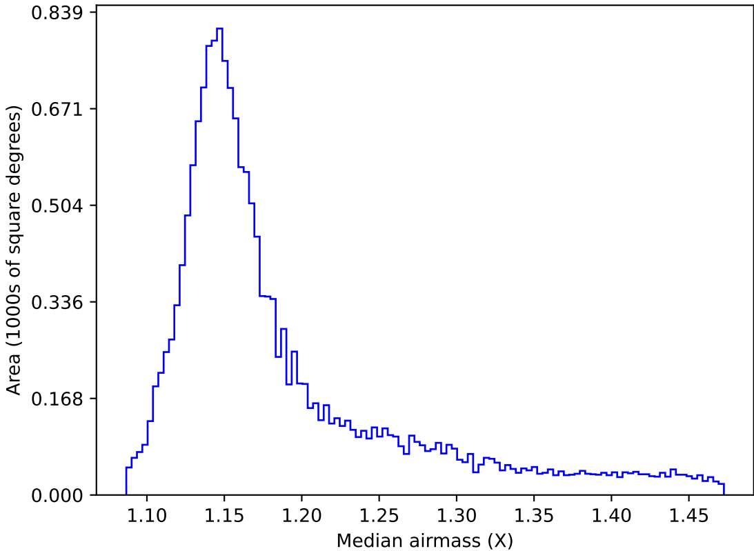
ddf_acor_sf25_lsf40_lsr10_v3.4_10yrs WFD y band: Median airmass
