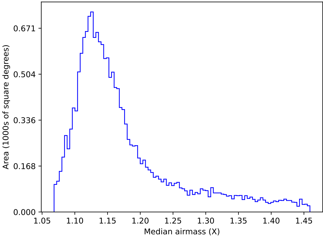
ddf_acor_sf25_lsf40_lsr10_v3.4_10yrs WFD u band: Median airmass
