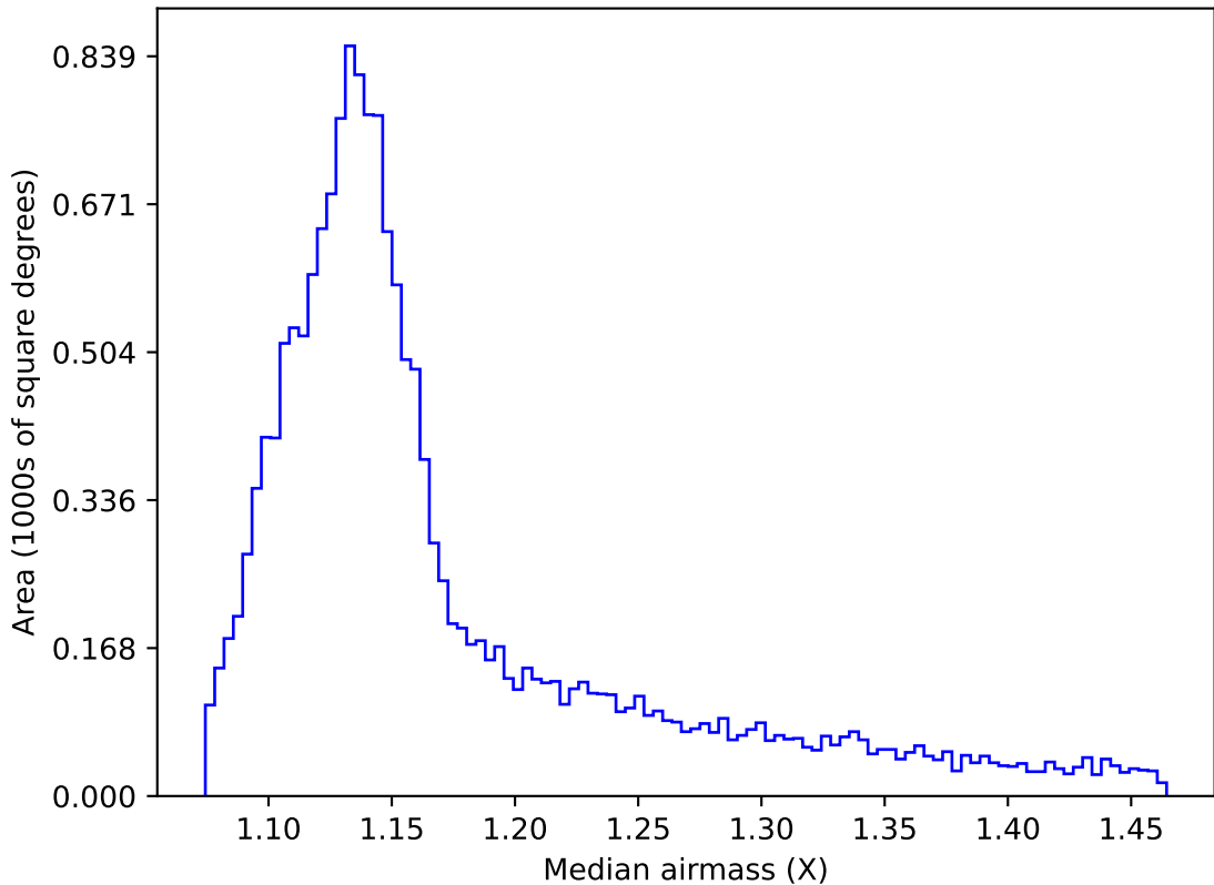
ddf_acor_sf25_lsf40_lsr10_v3.4_10yrs WFD r band: Median airmass
