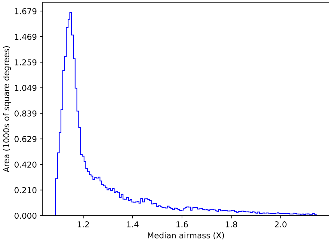
ddf_acor_sf25_lsf40_lsr10_v3.4_10yrs All sky z band: Median airmass
