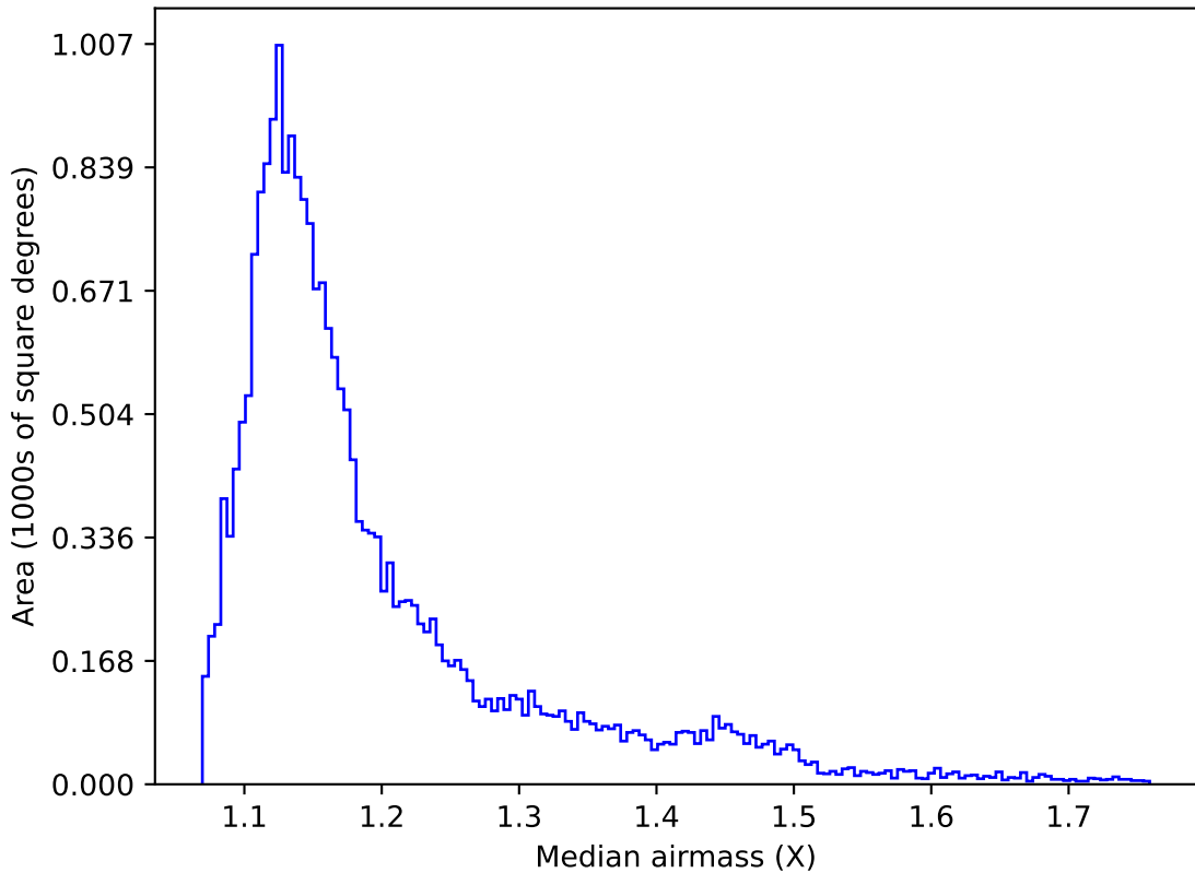
ddf_acor_sf25_lsf40_lsr10_v3.4_10yrs All sky u band: Median airmass
