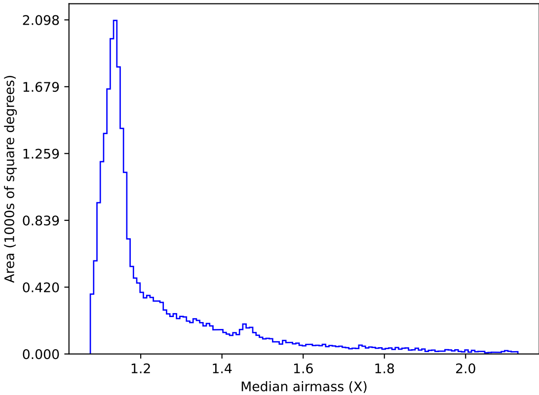
ddf_acor_sf25_lsf40_lsr10_v3.4_10yrs All sky r band: Median airmass
