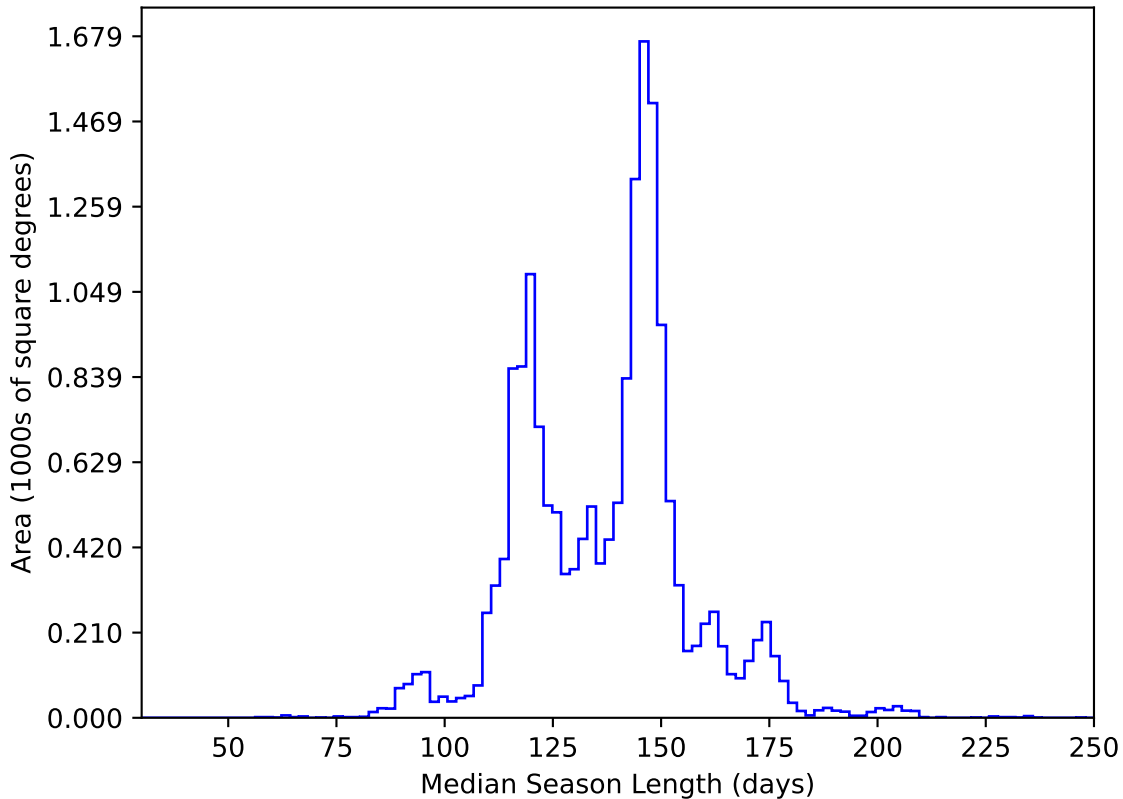
ddf_acor_sf25_lsf40_lsr10_v3.4_10yrs WFD y band: Median Season Length
