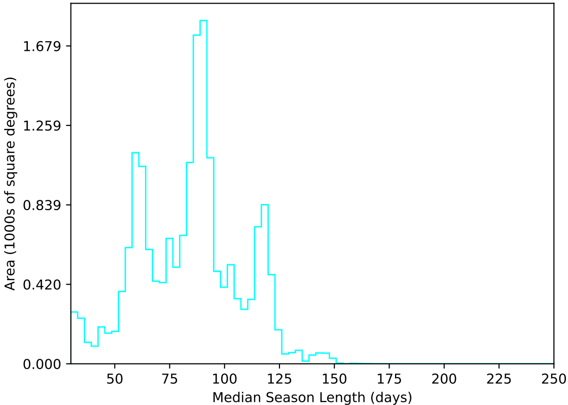
ddf_acor_sf25_lsf40_lsr10_v3.4_10yrs WFD u band: Median Season Length
