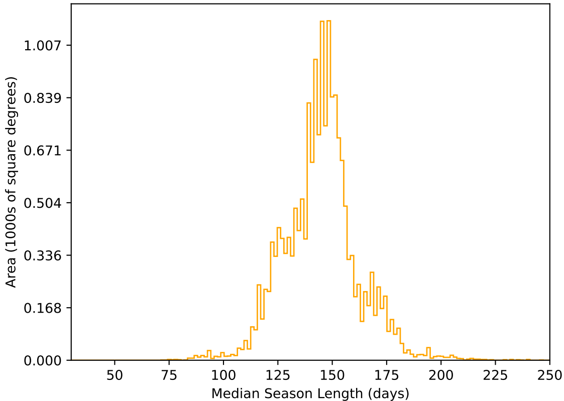
ddf_acor_sf25_lsf40_lsr10_v3.4_10yrs WFD r band: Median Season Length
