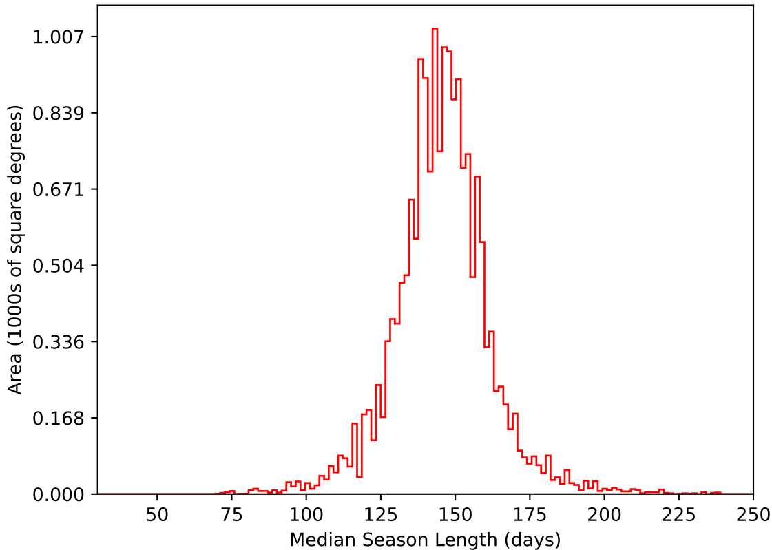
ddf_acor_sf25_lsf40_lsr10_v3.4_10yrs WFD i band: Median Season Length
