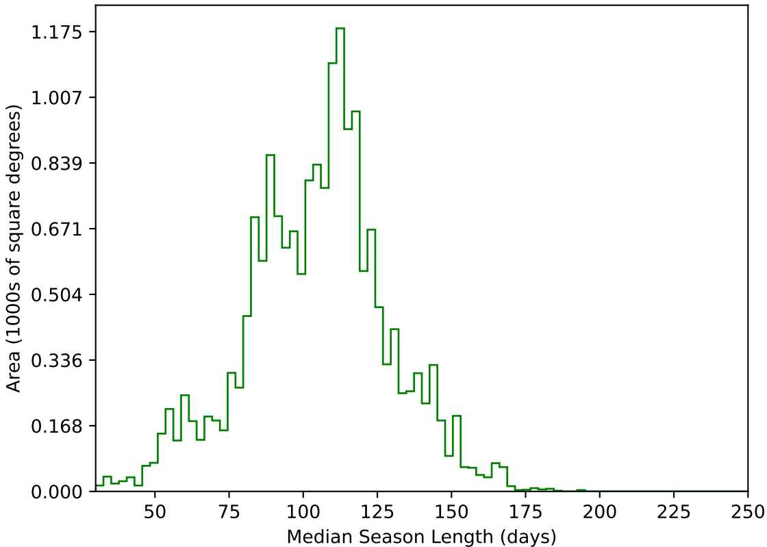
ddf_acor_sf25_lsf40_lsr10_v3.4_10yrs WFD g band: Median Season Length
