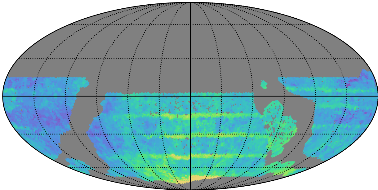
ddf_acor_sf25_lsf40_lsr10_v3.4_10yrs WFD all bands: Median Season Length
