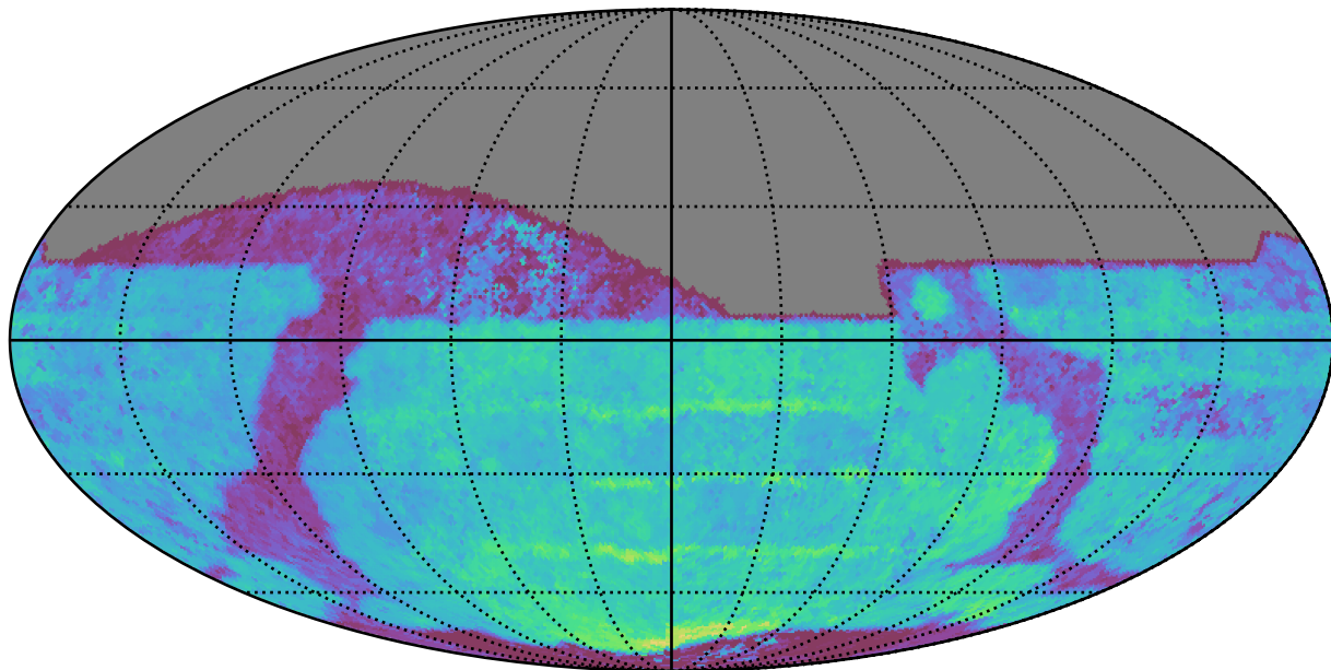
ddf_acor_sf25_lsf40_lsr10_v3.4_10yrs All sky z band: Median Season Length
