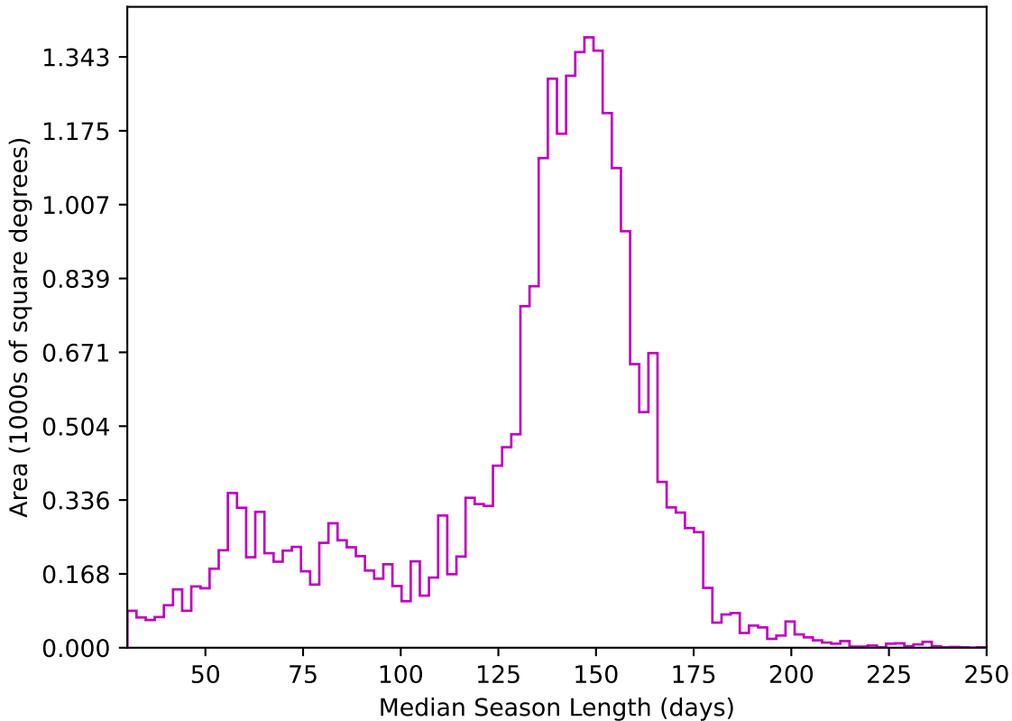
ddf_acor_sf25_lsf40_lsr10_v3.4_10yrs All sky z band: Median Season Length
