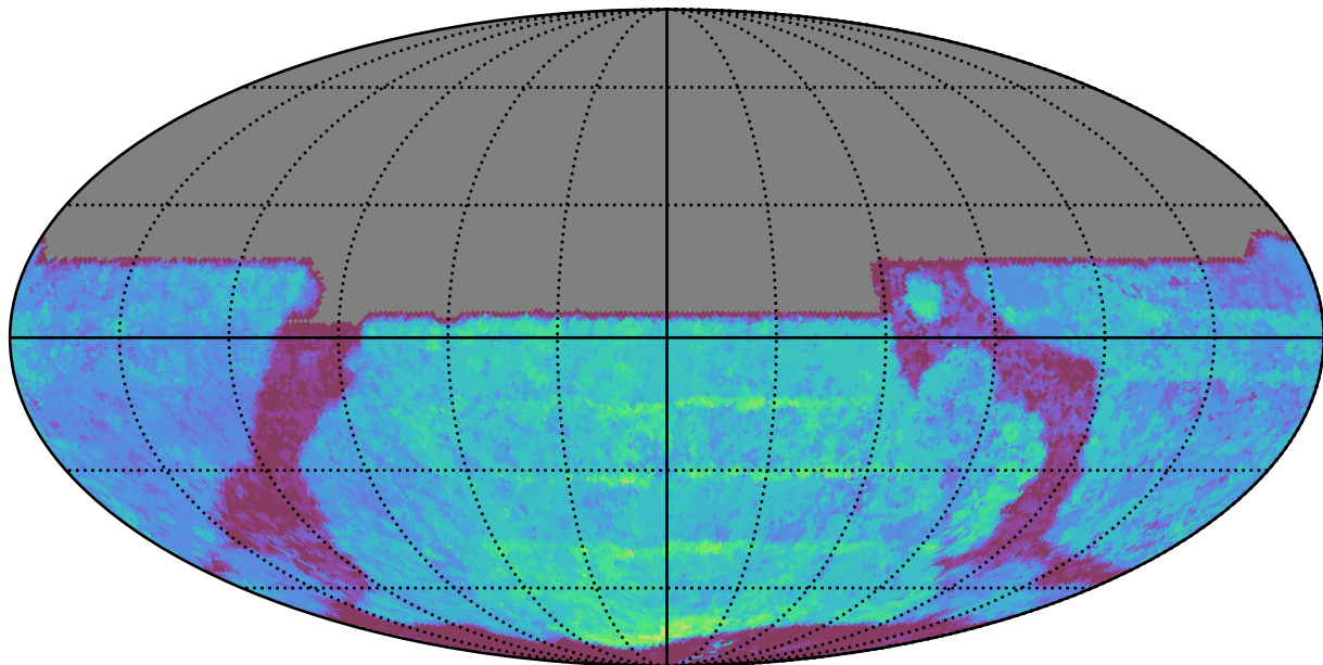
ddf_acor_sf25_lsf40_lsr10_v3.4_10yrs All sky y band: Median Season Length
