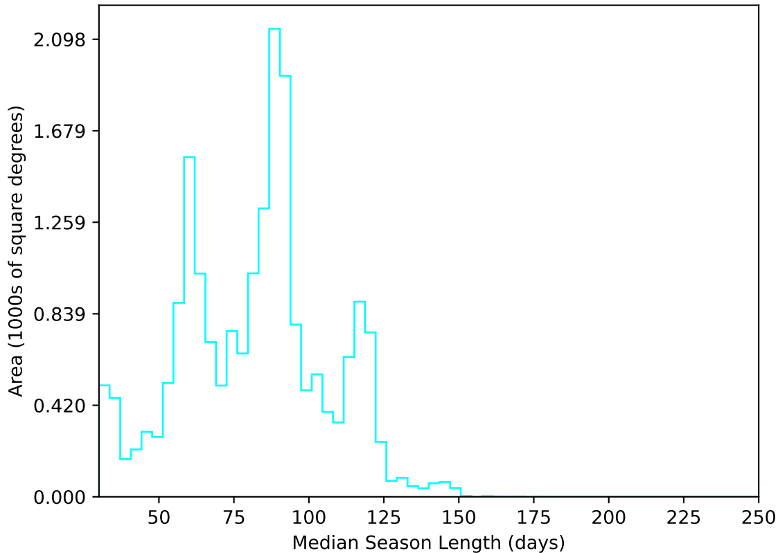
ddf_acor_sf25_lsf40_lsr10_v3.4_10yrs All sky u band: Median Season Length
