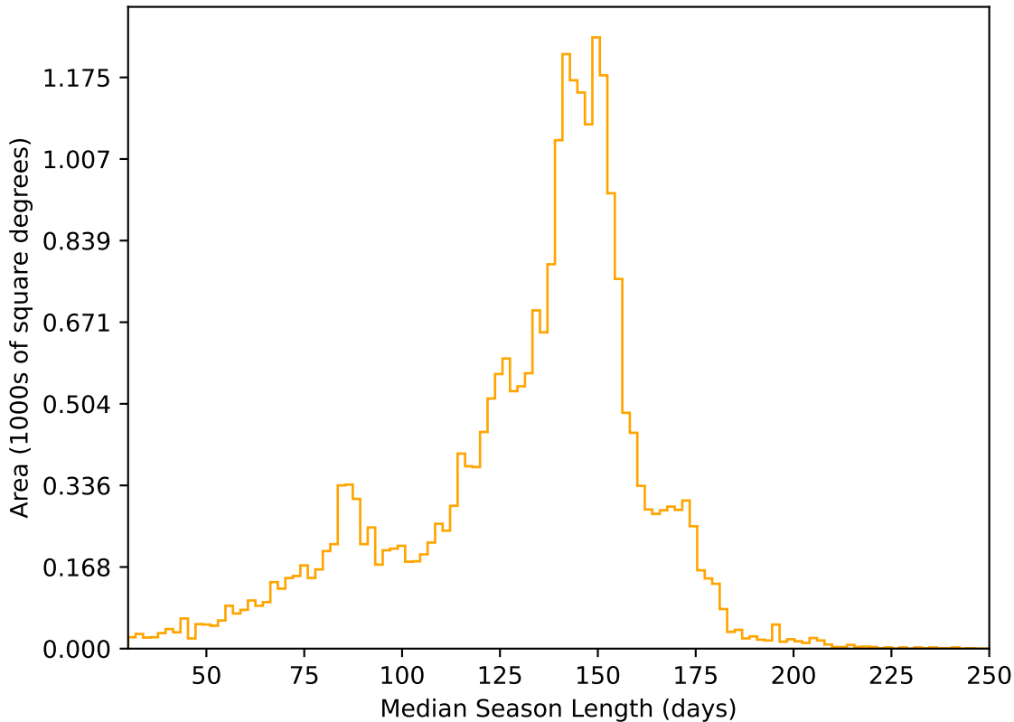
ddf_acor_sf25_lsf40_lsr10_v3.4_10yrs All sky r band: Median Season Length
